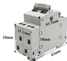
2M 36mm Width
