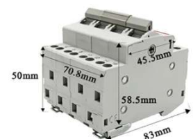
4M 72mm Width
